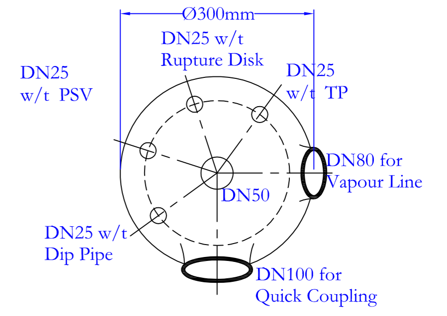
Top View for 300DN Glass Cover
