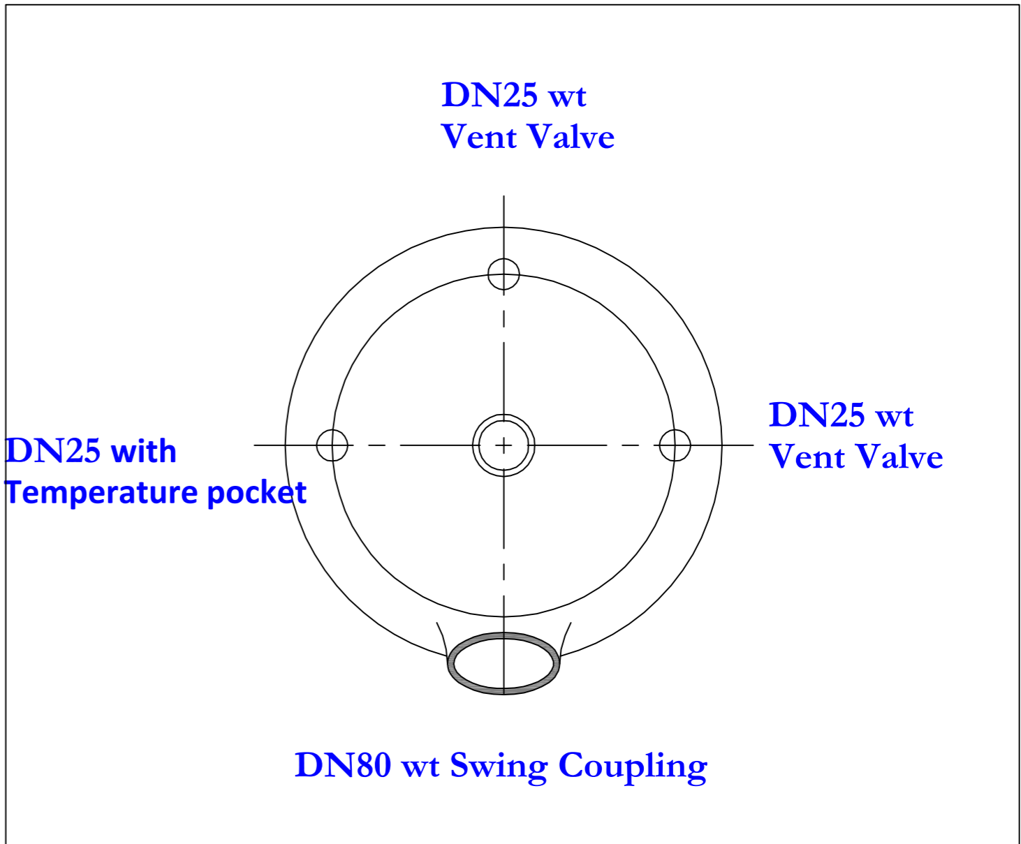
TOP VIEW OF 10 LTR SPHERICAL VESSEL
